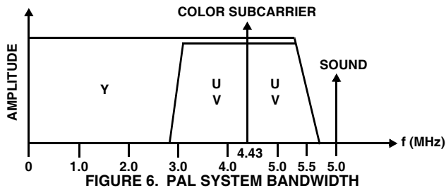
FIGURE 6. PAL SYSTEM BANDWIDTH
